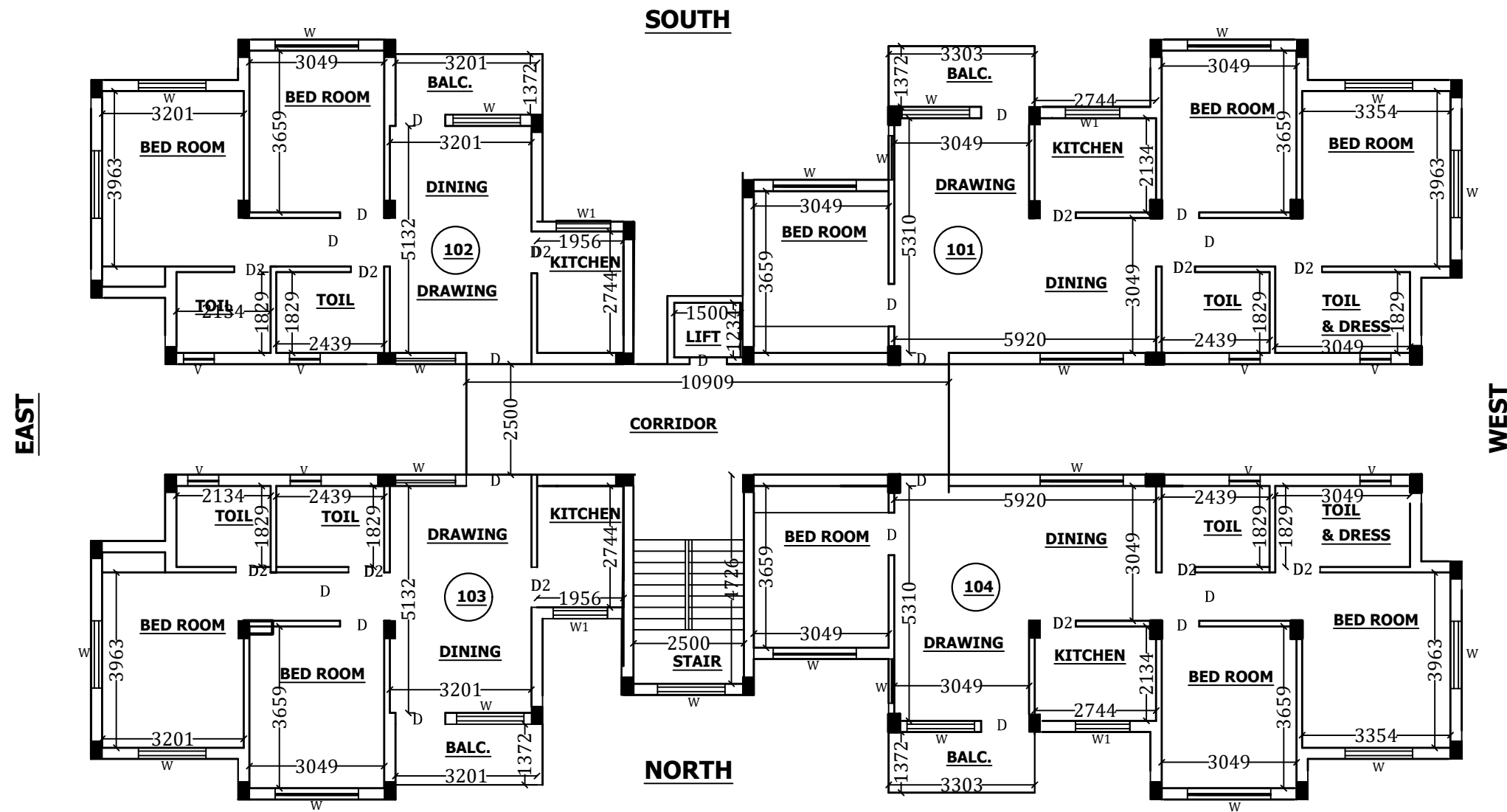
FIRST TO FOURTH FLOOR SAME (BLOCK -D)
